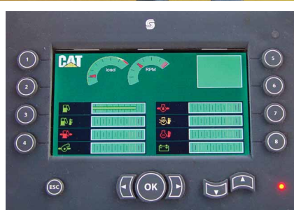
The large display provides operating parameters for machine and engine diagnostics. (Optional color display shown at left.)
