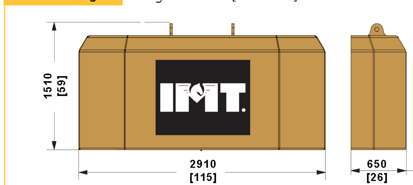
Counterweight Weight = 8 ton [17637 lb]
