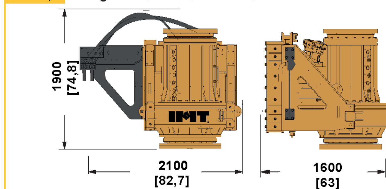
Rotary Weight = 4,7 ton [10300 lb]
